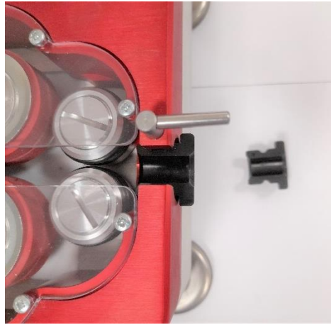
Figure 17: Open the cable entry adapter kit turning the lever outwards
