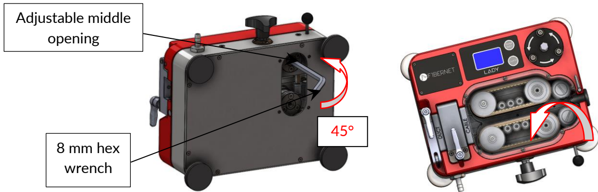
Figure 28: necessary steps to remove the drive belts.
