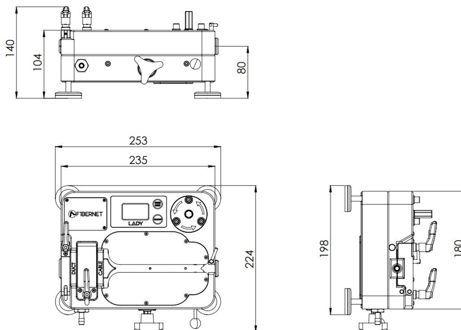
Figure 2: Lady – External dimensions.
