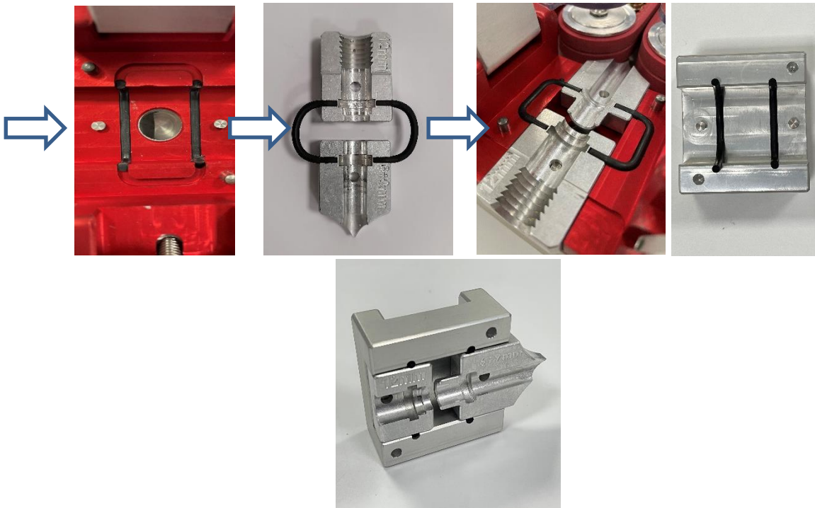
Figure 32: mounting the new gaskets.
