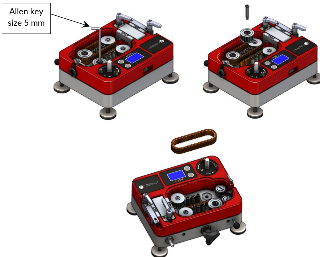
Figure 29: extracting the drive belt.
