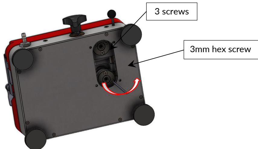
Figure 27: three hex screws to loosen up
