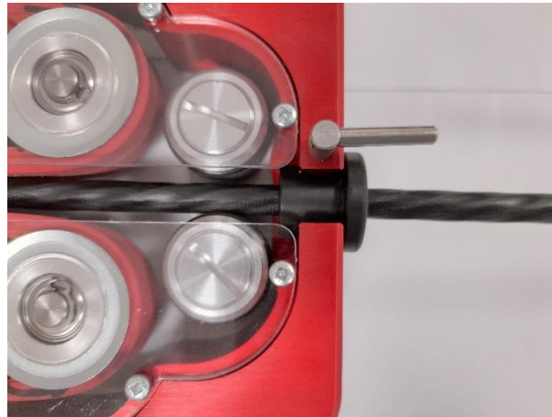
Figure 22: cable insertion inside cable adapter kit.
