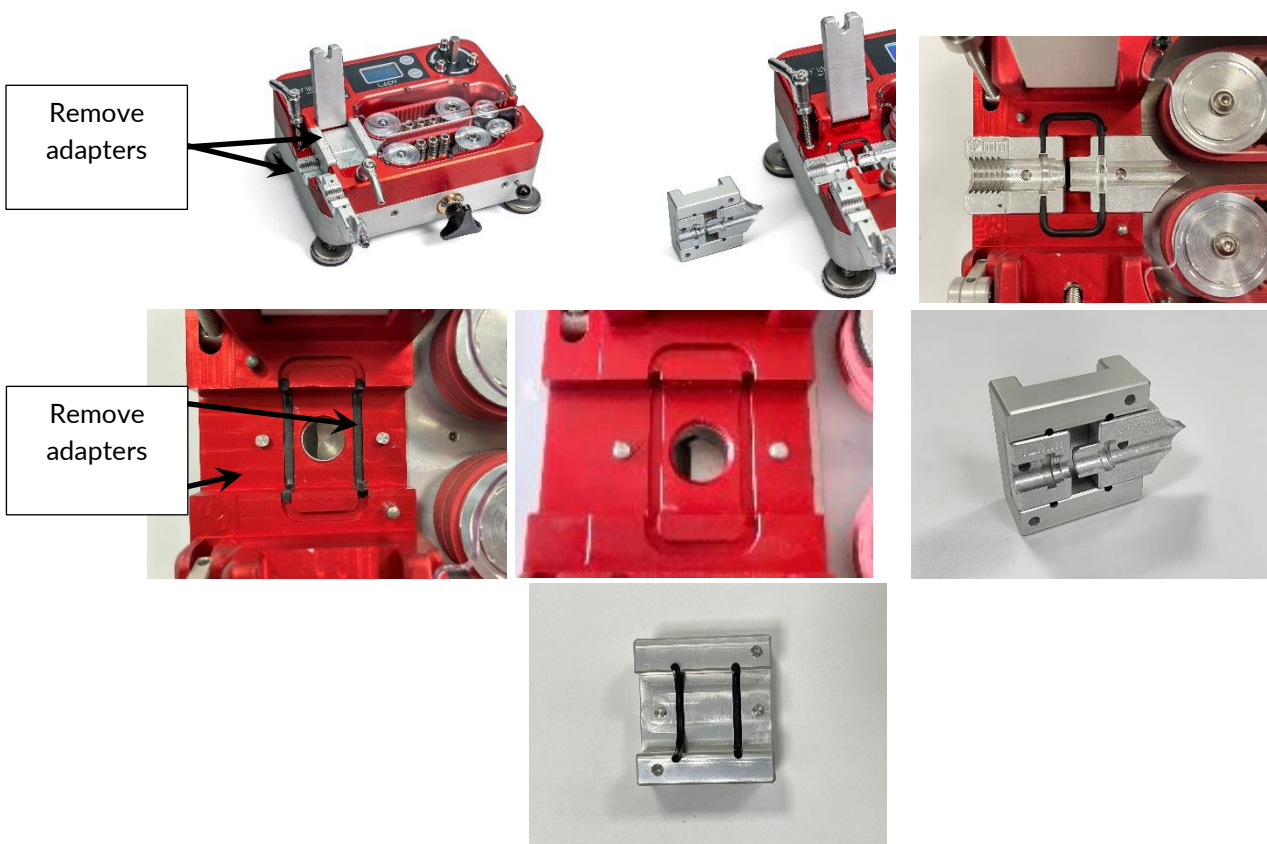
Figure 30: Unmounting adapters to remove gaskets
